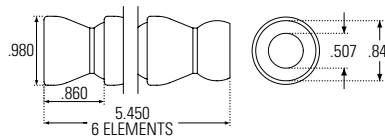
1/2" SYSTEM
