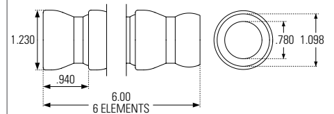
3/4" SYSTEM
