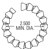
1/4" SYSTEM
