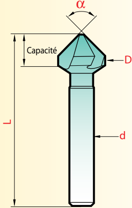
COUNTERSINK CHAMFER
